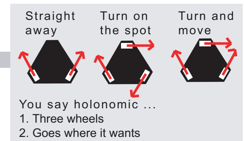
Omnidirectional wheels
